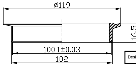
4" weld ferrule
