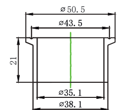
1.5" weld ferrule
