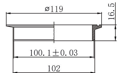
4" weld ferrule
