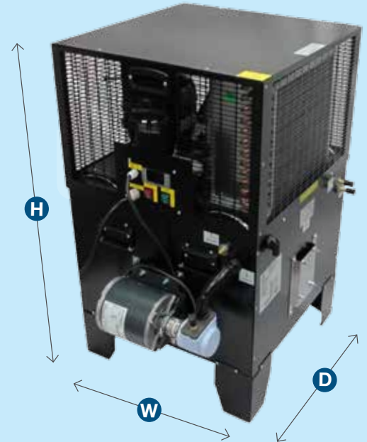
EXTRA 1/2 GP (Rotary Vane Pump)
